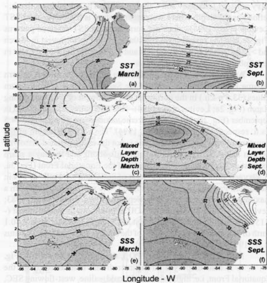
Figure 2. Environmental variables on the Eastern Equatorial Pacific Ocean: (a) sea-surface temperature (SST) in March, (b) SST in September, (c) mixed-layer depth (m) for March, (d) mixed-layer depth (m) for September, (e) sea-surface salinity (SSS) for March, (f) SSS for September. Data from Levitus et al. (1994).
