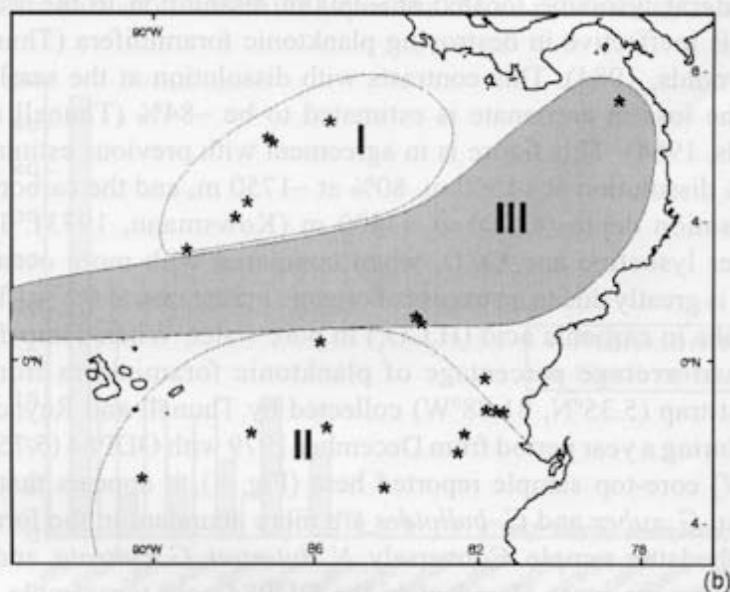
Figure 7. Core-top planktonic foraminiferal cluster analyses (UPGMA) for the Eastern Pacific; (a) dendrogram, (b) bioprovinces map. Core-top locations in asterisks.
