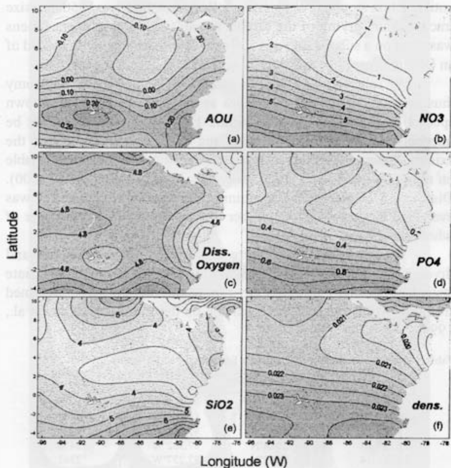
Figure 3. Environmental variables on the Eastern Equatorial Pacific Ocean: (a) Apparent oxygen utilization (AOU), (b) nitrate ( \text{NO}_3 ) in mmol, (c) dissolved oxygen in ml/l, (d) phosphate ( \text{PO}_4 ) in mmol, (e) silica ( \text{SiO}_2 ) in mmol and, (f) density. Data from Levitus et al. (1994).
