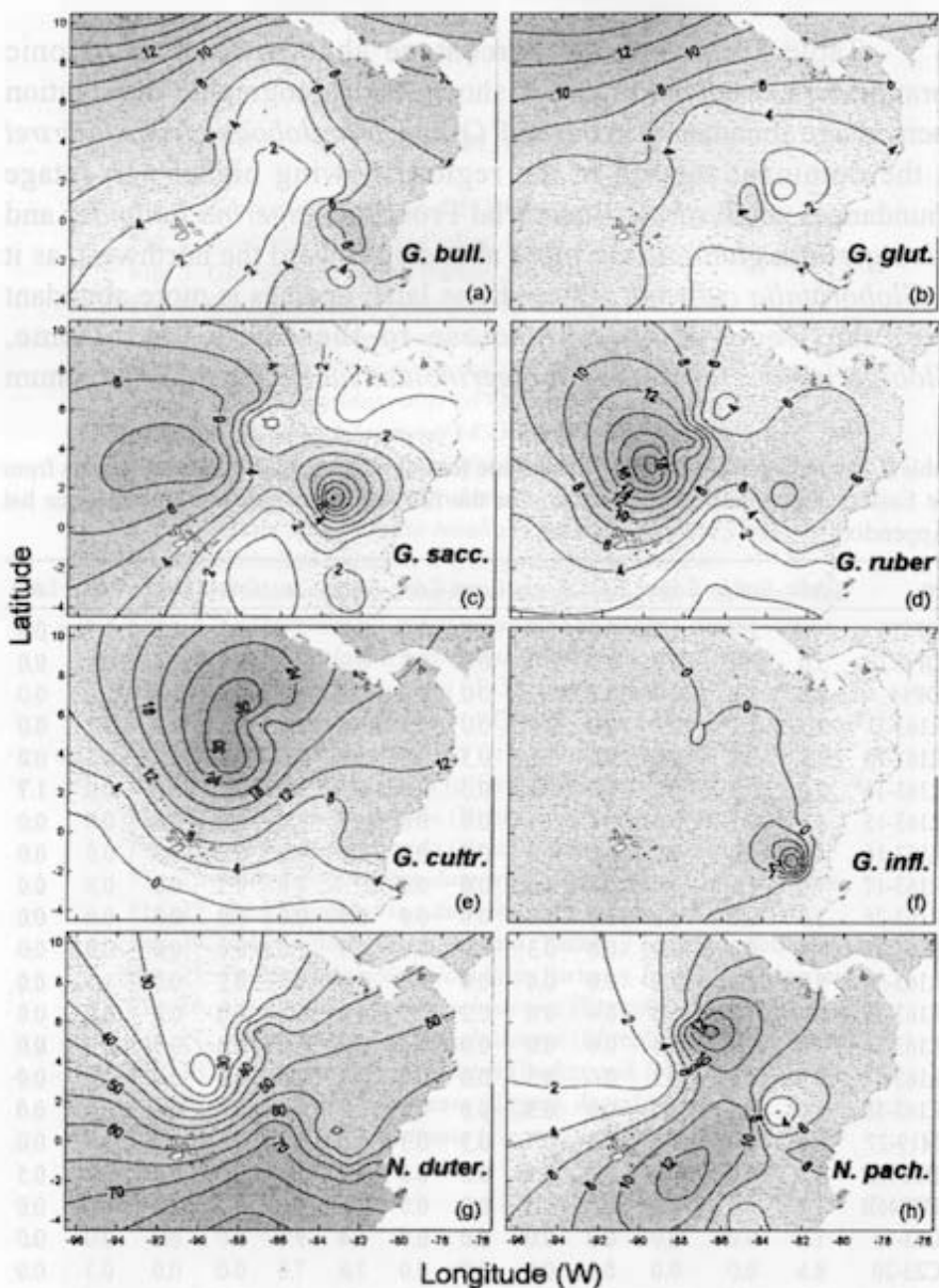
Figure 4. Relative abundance (percentage) of planktonic foraminifera in core-top from the Eastern Pacific: (a) Globigerina bulloides , (b) Globigerinina glutinata , (c) Globigerinoides sacculifer , (d) Globigerinoides ruber , (e) Globorotalia cultrata , (f) Globorotalia inflata , (g) Neogloboquadrina dutertrei , (h) Neogloboquadrina pachyderma .
