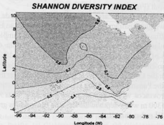
Figure 6. Shannon diversity index from core-top samples from the Eastern equatorial Pacific Ocean.
