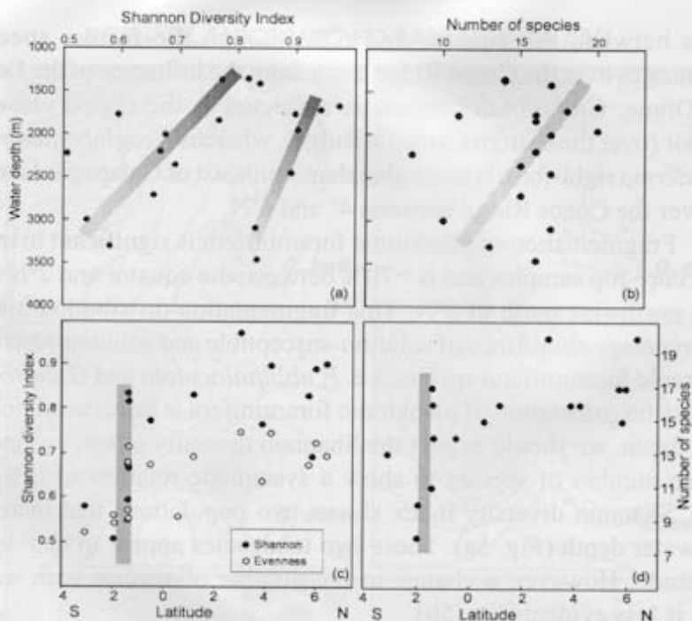
Figure 5. Core-top planktonic foraminiferal diversity for the Eastern Pacific: (a) Shannon diversity index and evenness against water depth, (b) number of species against water depth, (c) Shannon diversity index and evenness against latitude, (d) Number of species against latitude.
