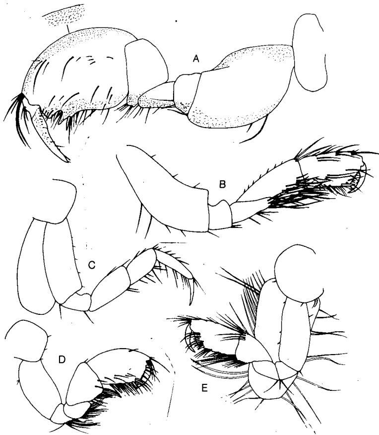
Fig. 23. Lembos scolosternum n.sp., A-C, male holotype, USNM 266452; D-E, female paratype, sta. LAB2, USNM 266453: A, gnathopod 1; B, gnathopod 2; C, pereopod 3; D, gnathopod 1; E, gnathopod 2.
